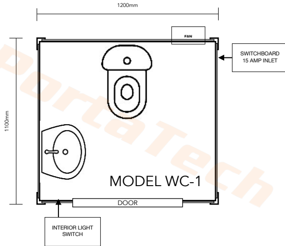
2022 PORTATECH WC-1 UNIT (ELECTRICAL INCLUSIVE) STEEL/EPS PANEL/FIBRE CEMENT STRUCTURE COLOUR: WHITE/WHITE
