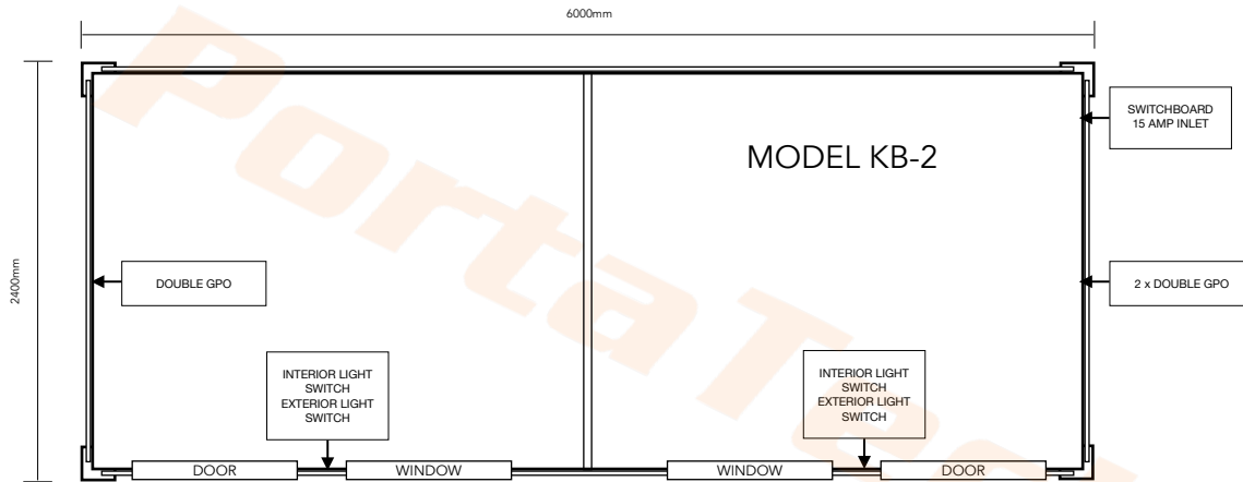
2022 PORTATECH KB-2 UNIT (ELECTRICAL INCLUSIVE) STEEL/EPS PANEL/FIBRE CEMENT STRUCTURE COLOUR: WHITE/WHITE
