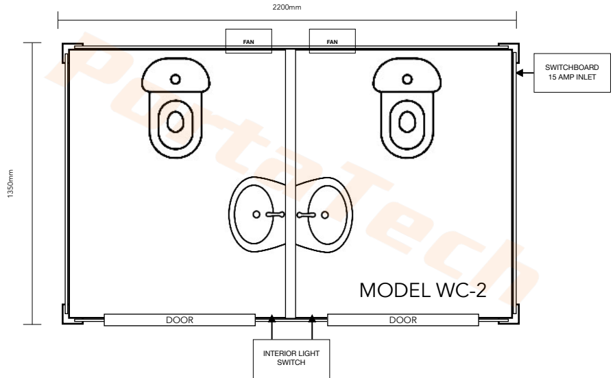
2022 PORTATECH WC-2 UNIT (ELECTRICAL INCLUSIVE) STEEL/EPS PANEL/FIBRE CEMENT STRUCTURE COLOUR: WHITE/WHITE
